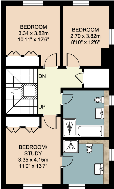
SECOND FLOOR
