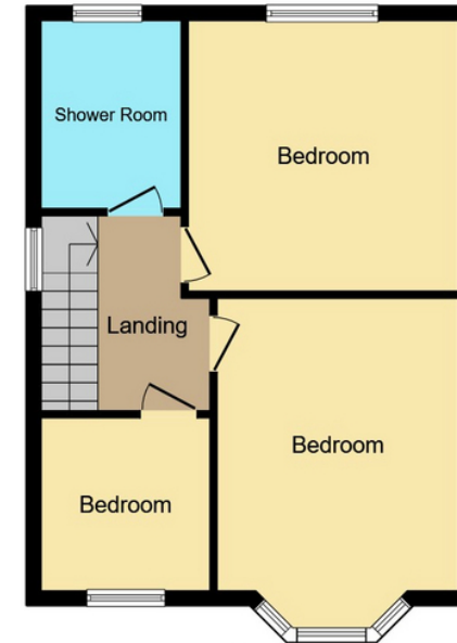
First Floor Floor area 47.9 m 2 (515 sq.ft.)
